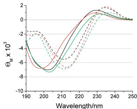
FIGURE 3: Conformational changes associated with protegrin variants binding to membranes. CD spectra of peptides: solid lines, peptides in the absence of lipid membranes; dashed lines, peptides in the presence of POPC/POPG (3:1); black lines, PG-1; red lines, PG-1-LL; green lines, PG-1-FF.
